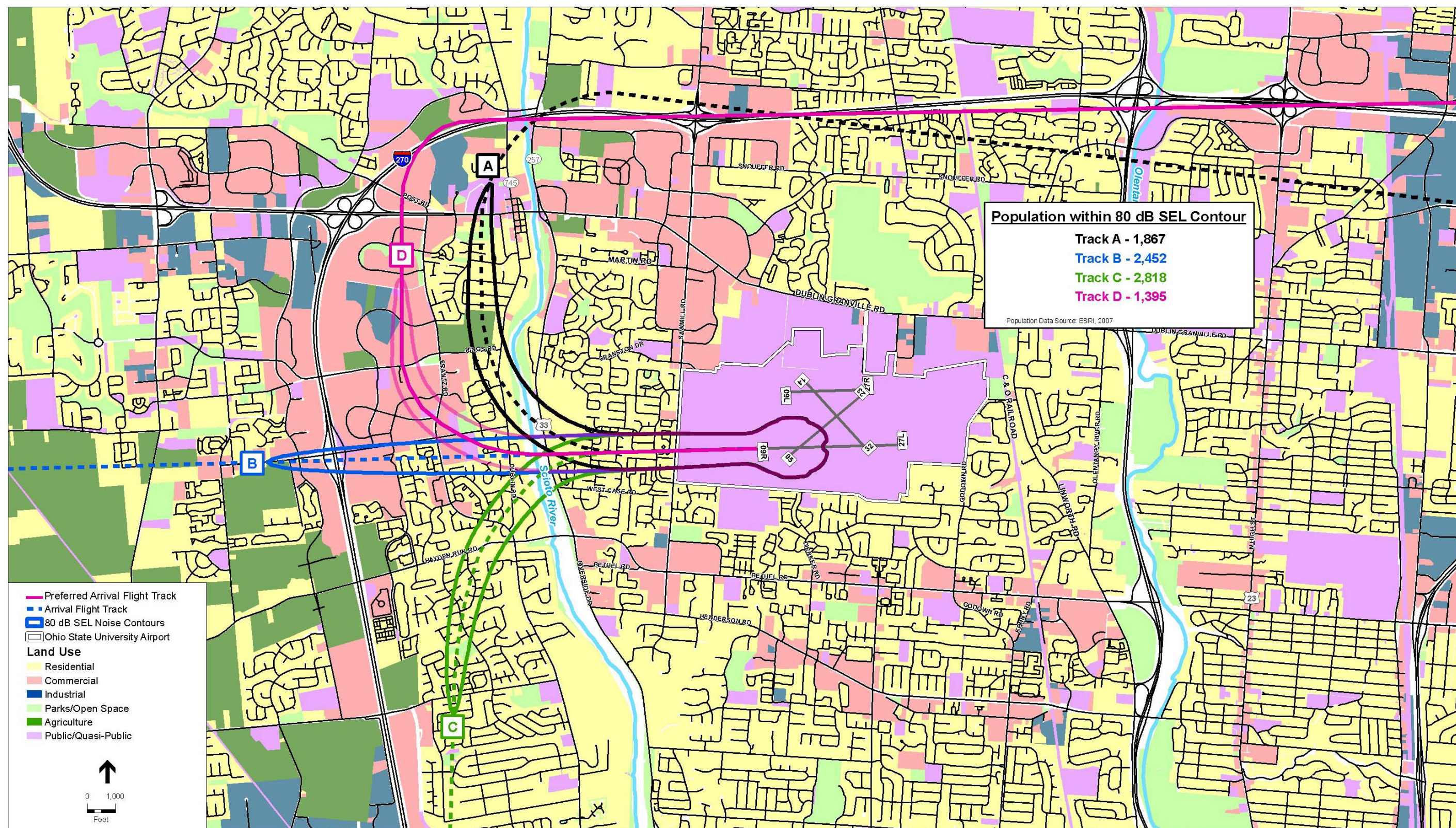
FIGURE 9-7 EXISTING JET AIRCRAFT ARRIVAL ANALYSIS – RUNWAY 9R
