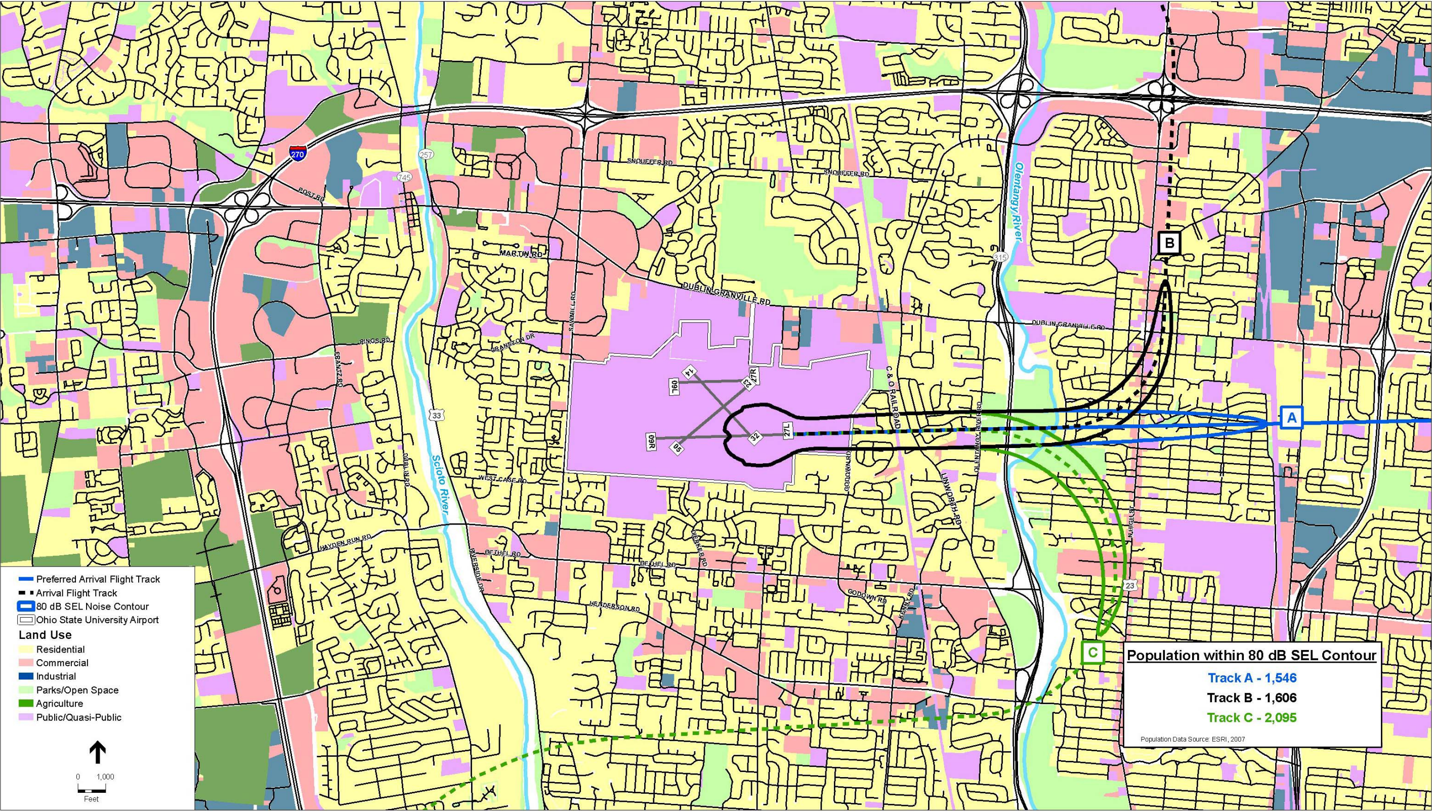
FIGURE 9-3 EXISTING JET AIRCRAFT ARRIVAL ANALYSIS – RUNWAY 27L
