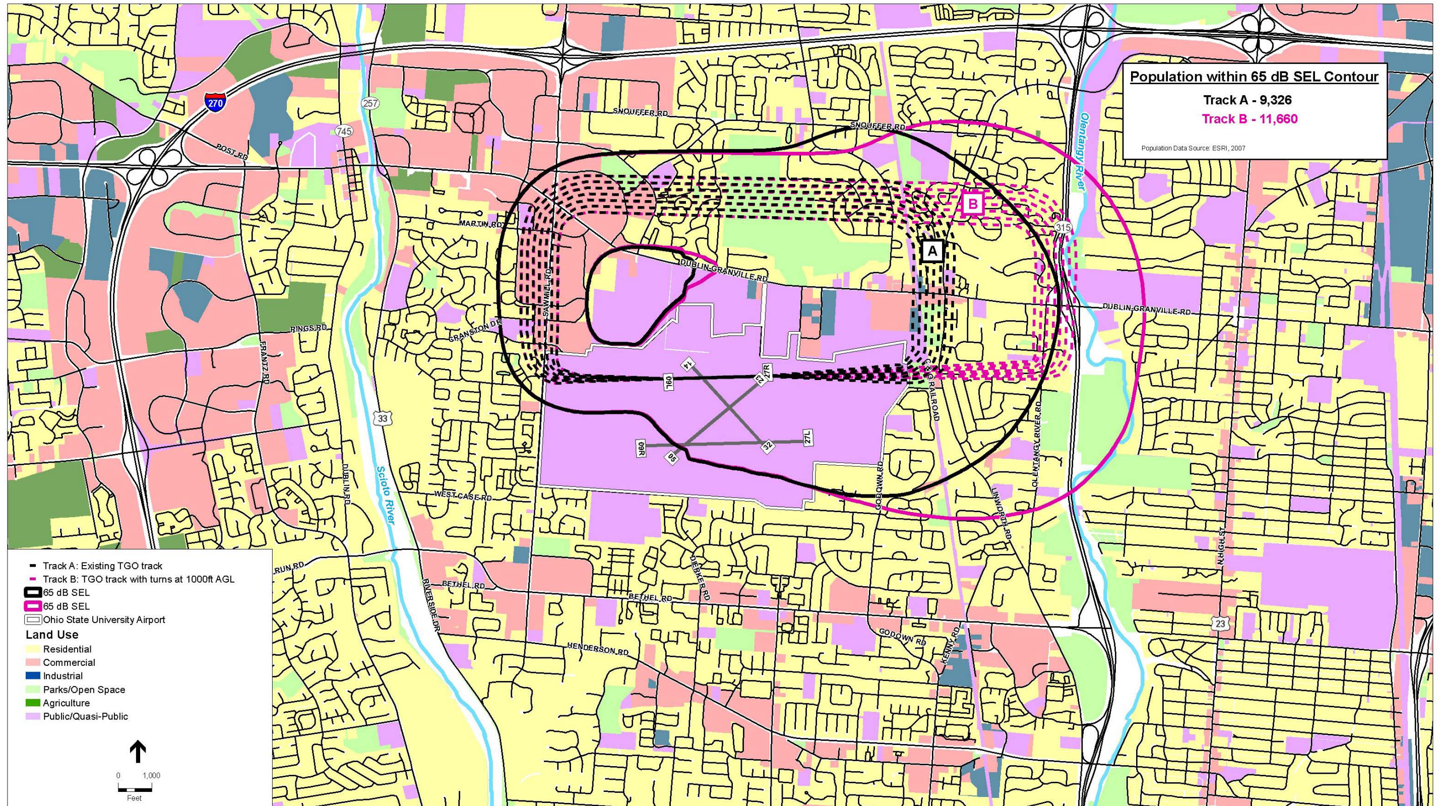
FIGURE 9-1 CNA172 SEL CONTOUR COMPARISON – EXISTING TRAINING PATTERN VS. ALTERNATIVE TRAINING PATTERN
