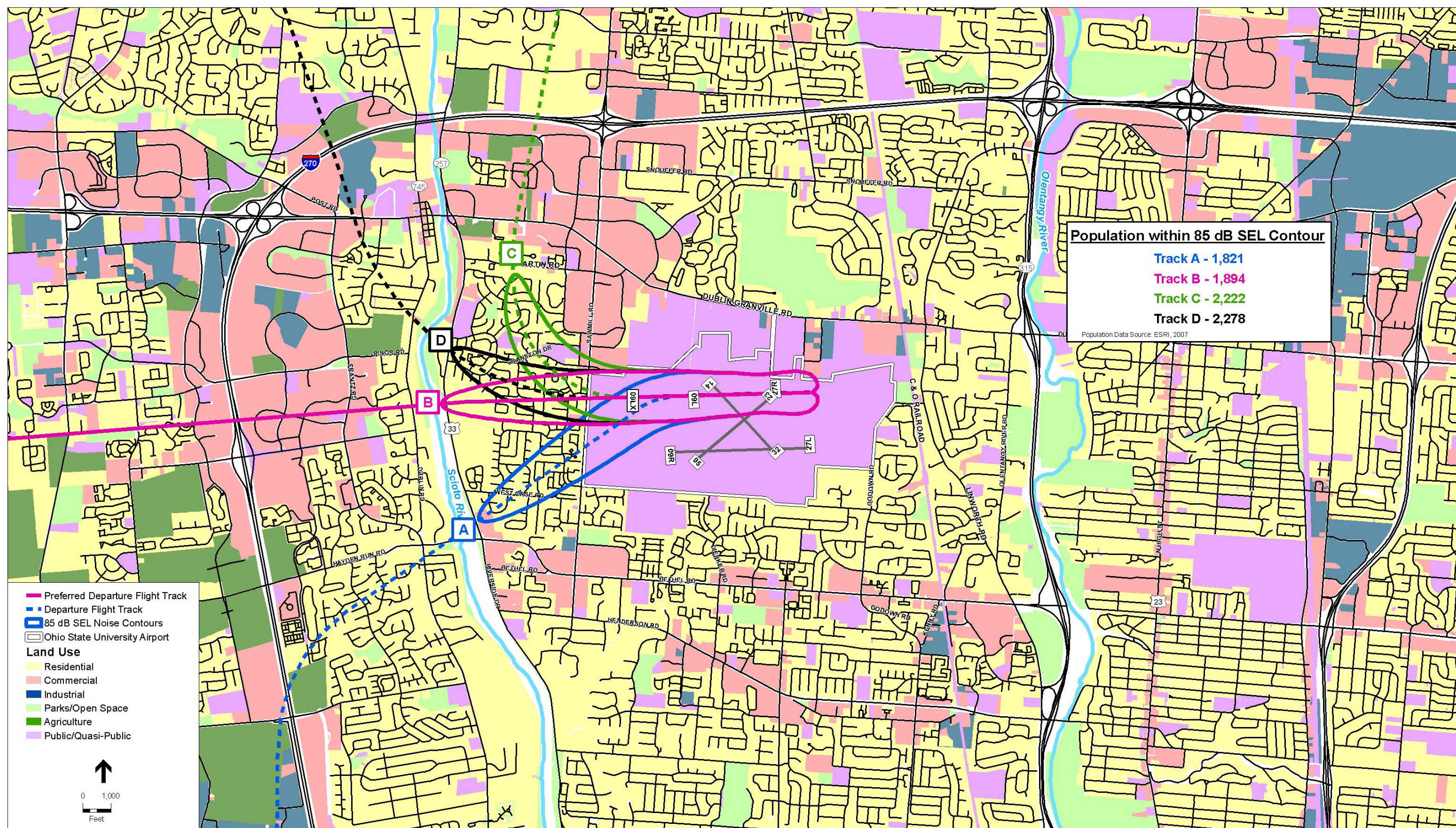
FIGURE 9-18 FUTURE PROPELLER AIRCRAFT DEPARTURE ANALYSIS – RUNWAY 27R
