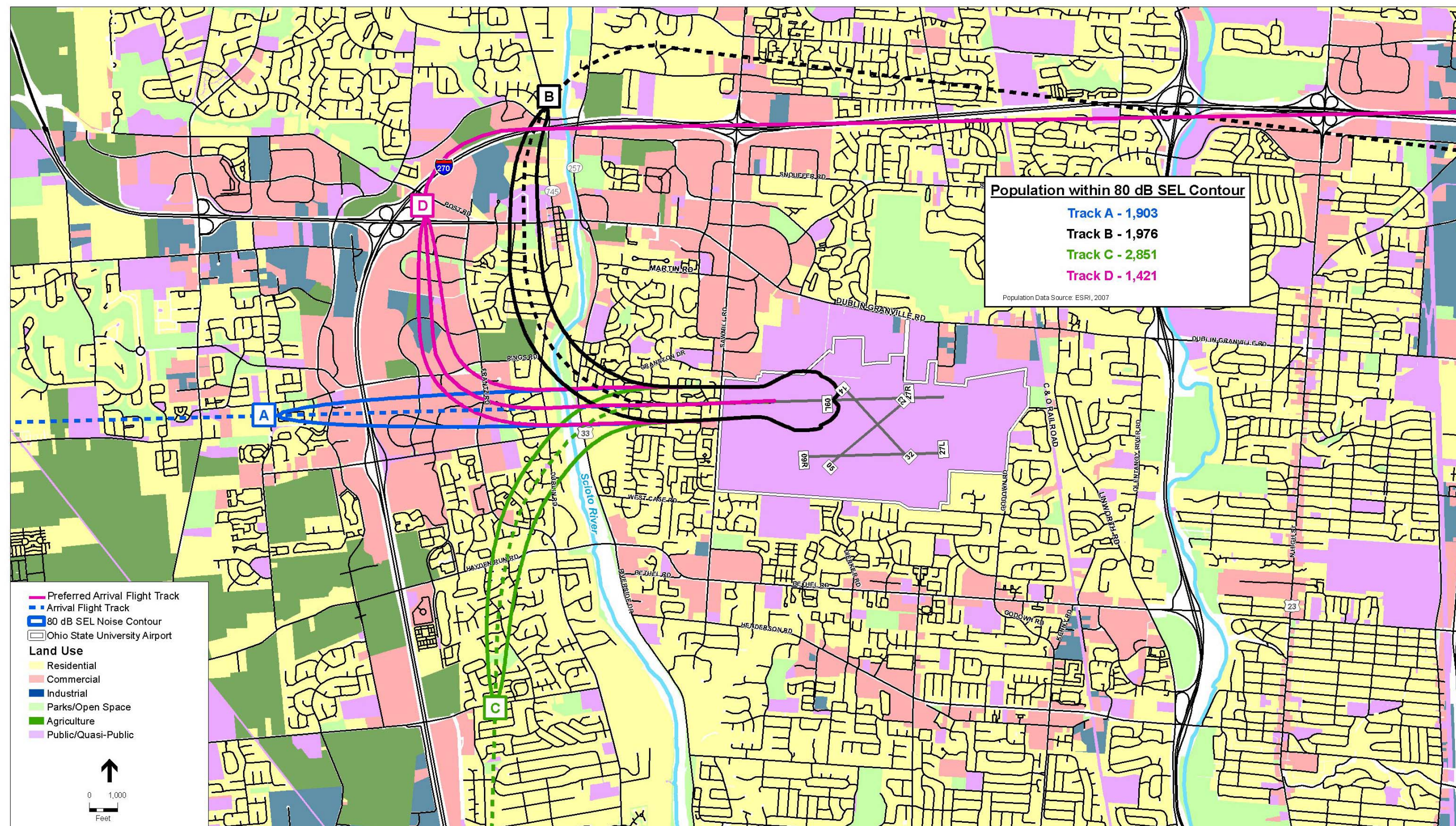
FIGURE 9-9 FUTURE JET AIRCRAFT ARRIVAL ANALYSIS – RUNWAY 9L
