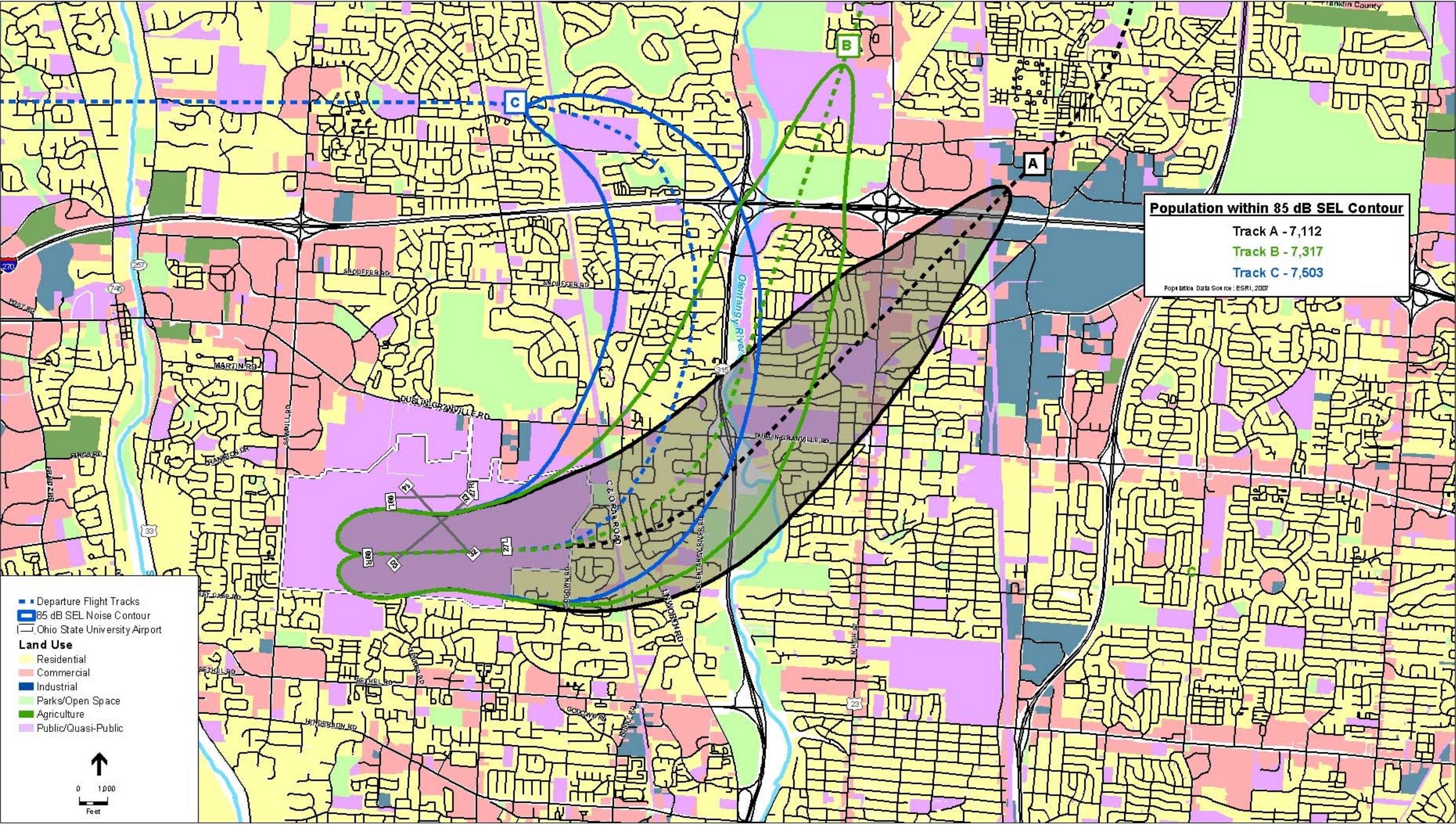
FIGURE 9-19 RUNWAY 9R JET ANALYSIS FOR 050 DEPARTURE HEADING
