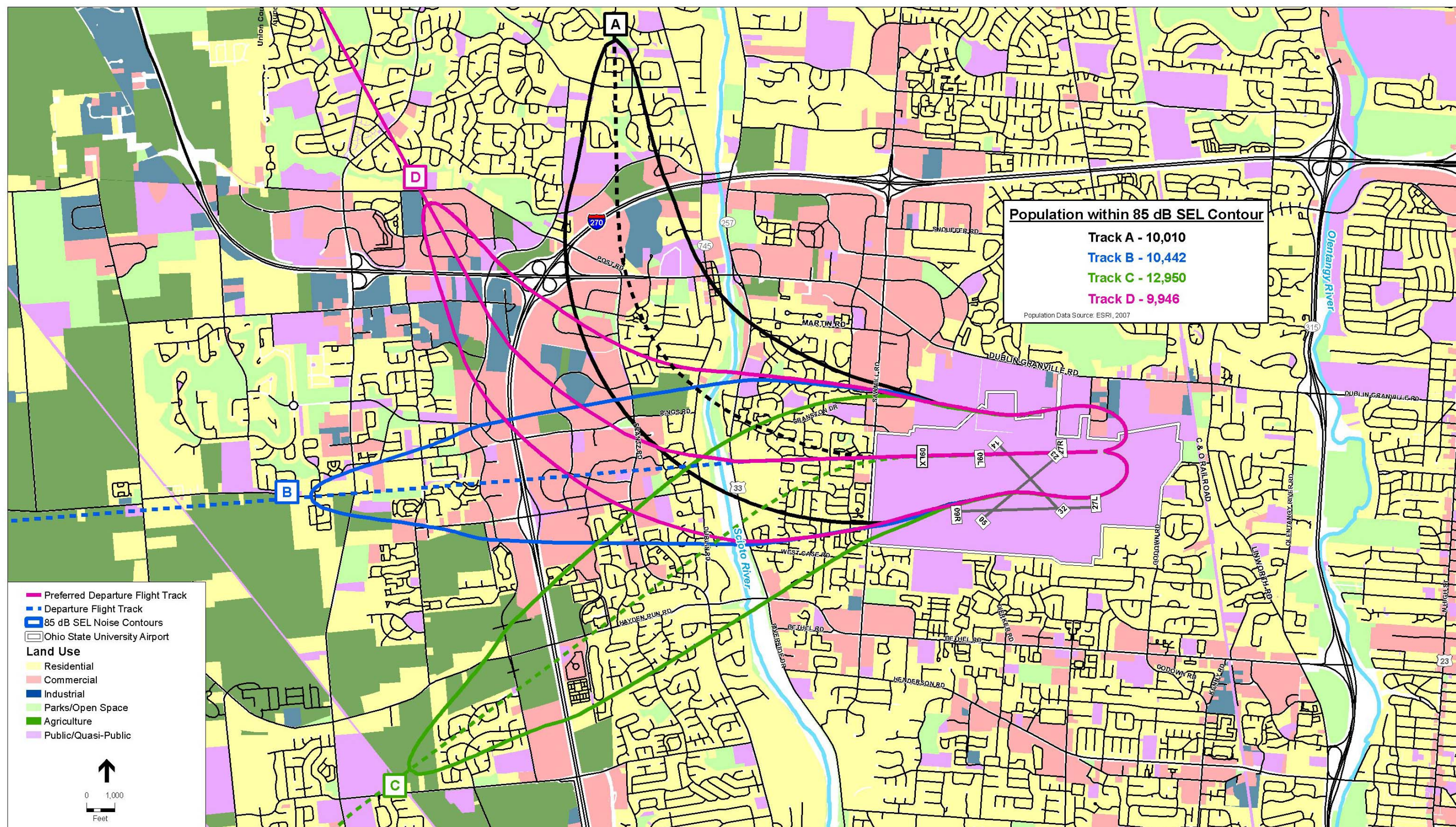
FIGURE 9-17 FUTURE JET AIRCRAFT DEPARTURE ANALYSIS – RUNWAY 27R
