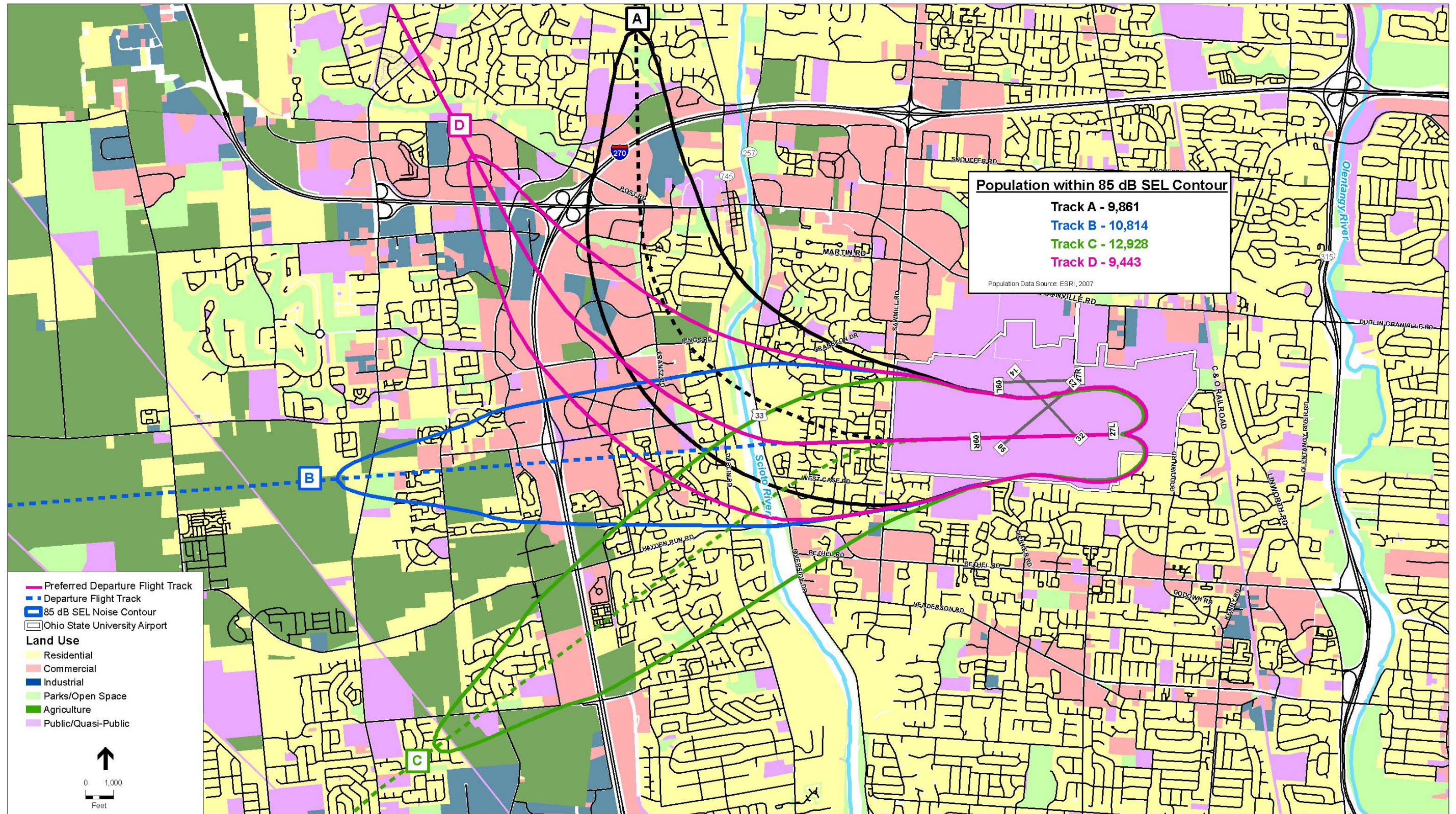
FIGURE 9-15 EXISTING JET AIRCRAFT DEPARTURE ANALYSIS – RUNWAY 27L
