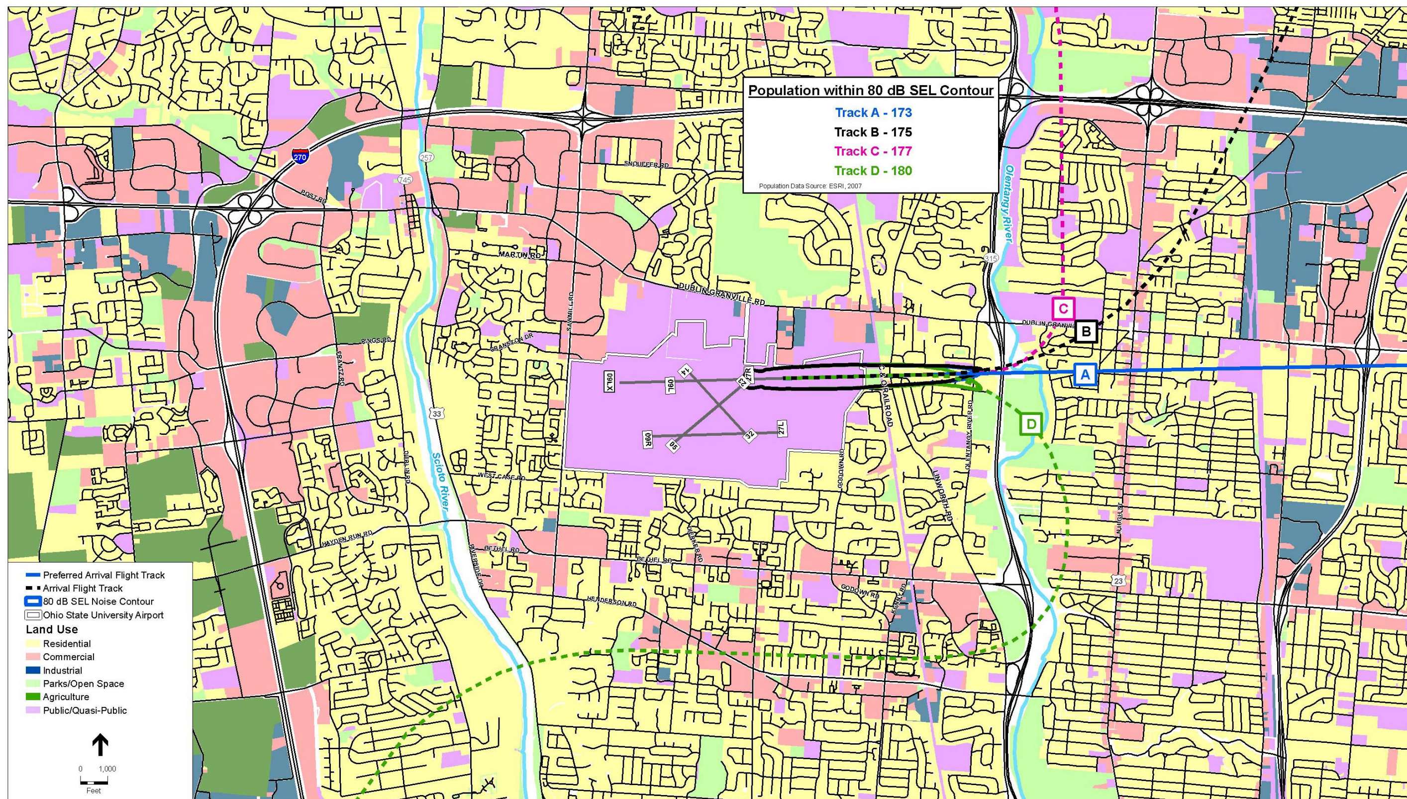
FIGURE 9-6 FUTURE PROPELLER AIRCRAFT ARRIVAL ANALYSIS – RUNWAY 27R
