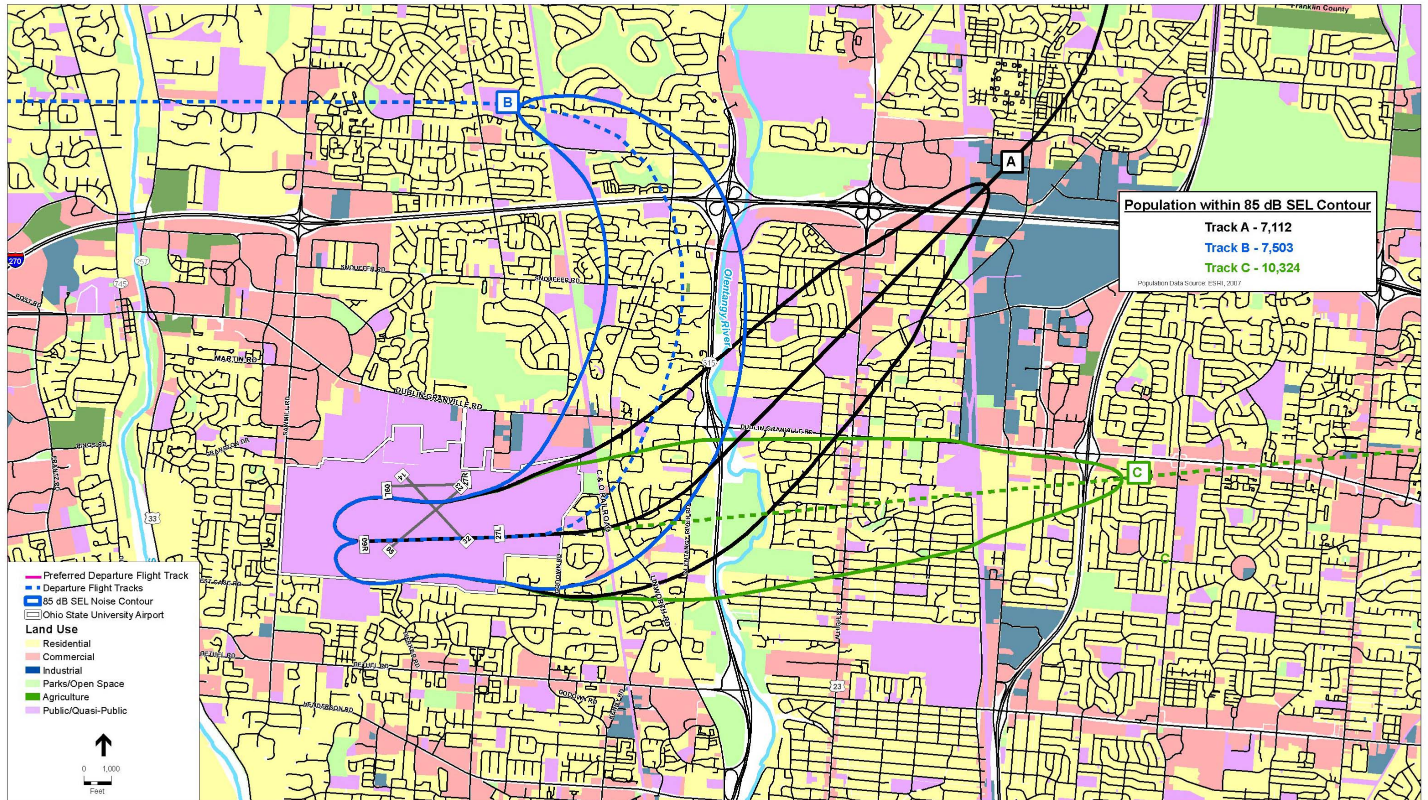
FIGURE 9-11 EXISTING JET AIRCRAFT DEPARTURE ANALYSIS – RUNWAY 9R
